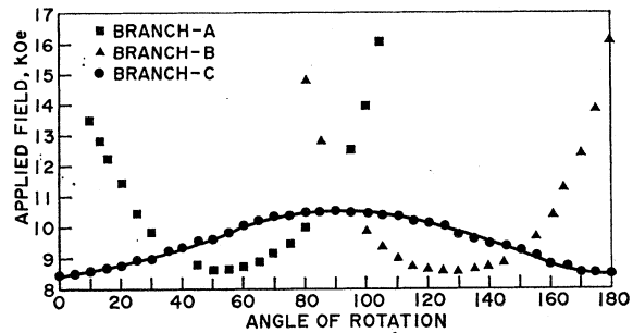
FIG. 7. Magnetic field for resonance as a function of crystallographic direction at the constant frequency 24 GHz. The sample is a single crystal with the magnetic field lying in a (110) plane. The solid curve is the result of fitting branch C to Eq. (29).
